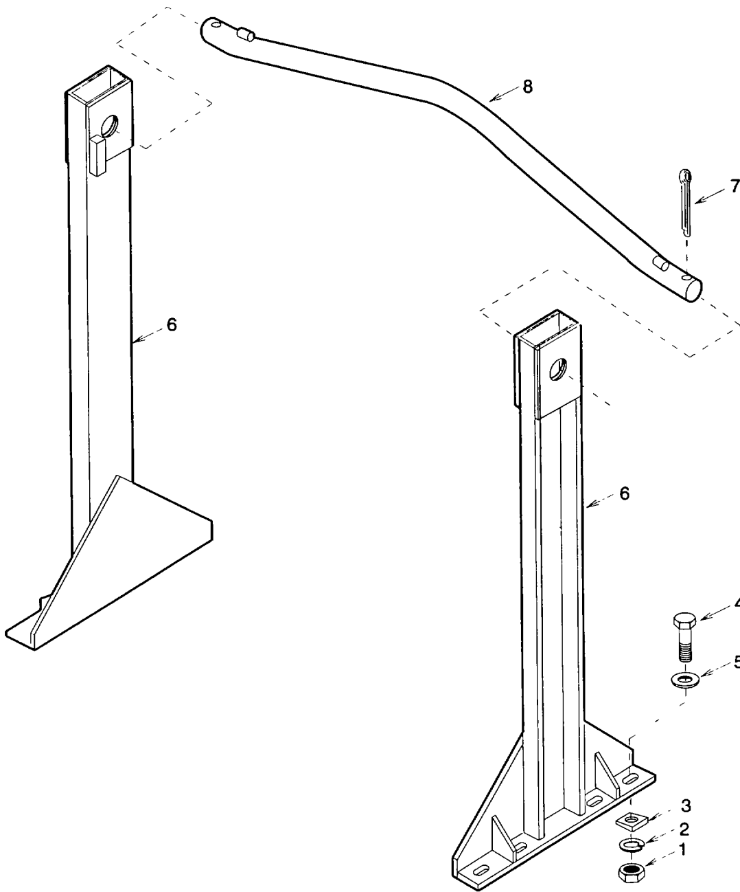
Figure 4-18. Lift Bar Assembly
