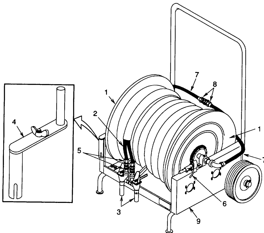
Figure 1-2. Location and Description of Major Components for the Auxiliary Mobile Hose Reel Cart
