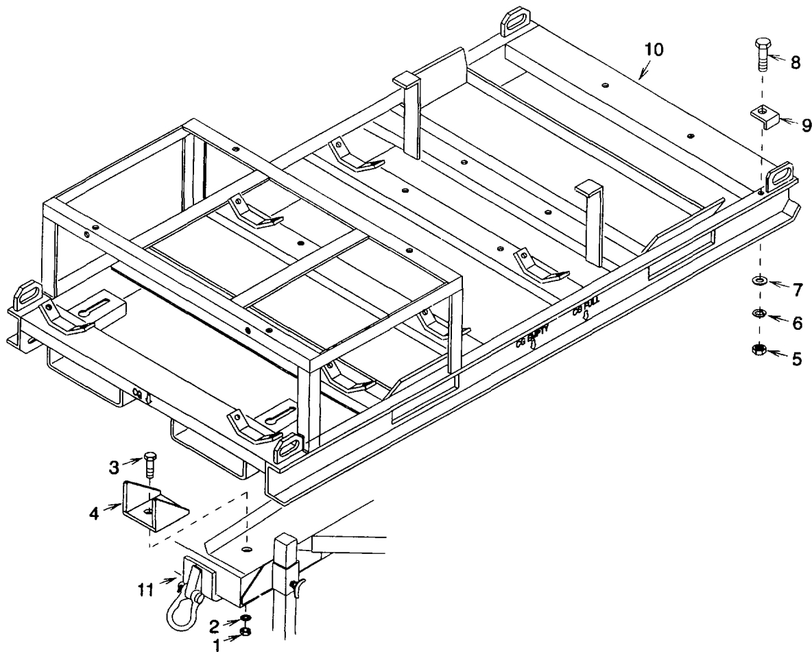
Figure 5-5. Skid Frame
