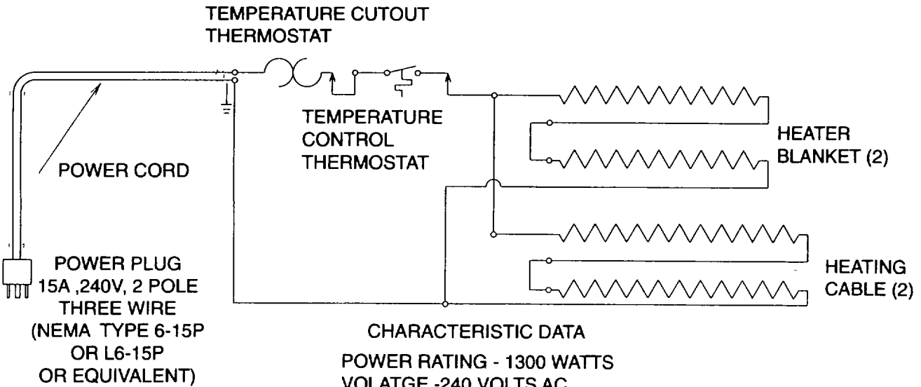
Figure 4-24. AFFF Tank Heater Electrical Schematic
